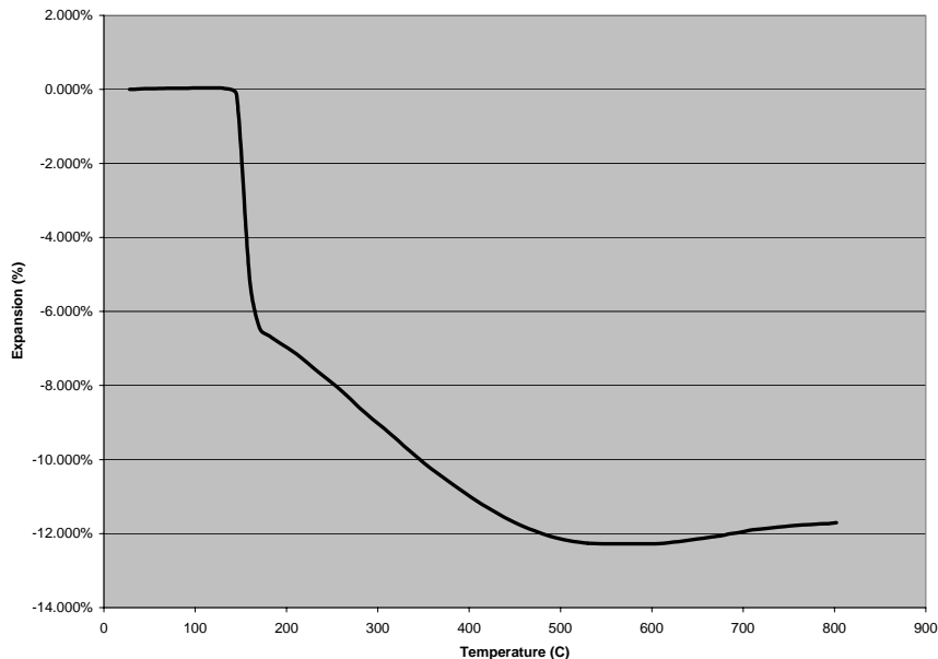
Ultra-fine S7000 TMA RT to 800C @ 10C/min in air
