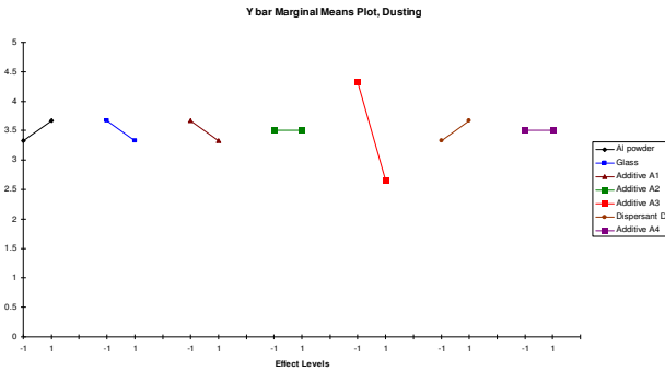
Figure 7 Marginal means plot showing extent of the effect of various factors on dusting
