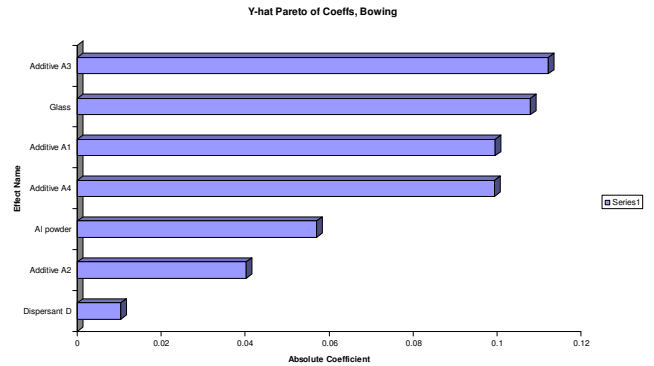
Figure 4 Pareto chart showing effect of 7 factors on bowing
