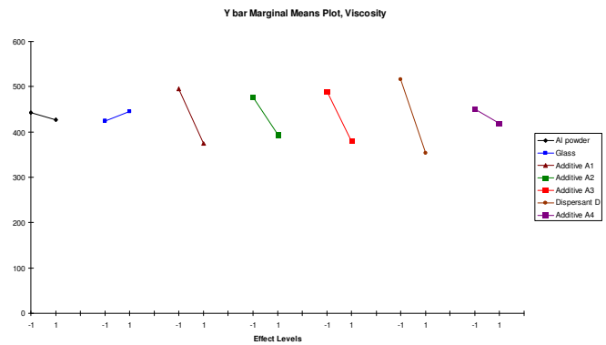
Figure 9 Marginal means plot showing effect of various factors on paste viscosity.
