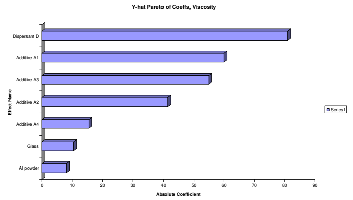
Figure 8 Pareto chart showing effect of various factors on viscosity of paste.
